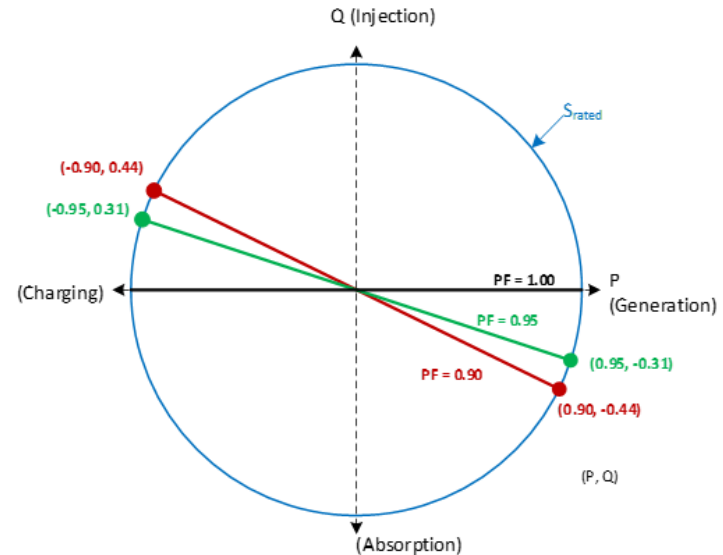
Figure 5—Constant power factor operation of ESS
